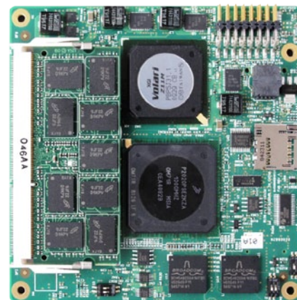
Figure 1: Emerson Network Power COM Express™ compatible module based on the QorIQ P2020 processor
